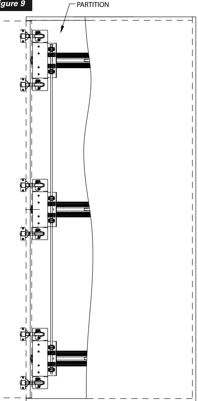
HINGE ADJUSTMENT
