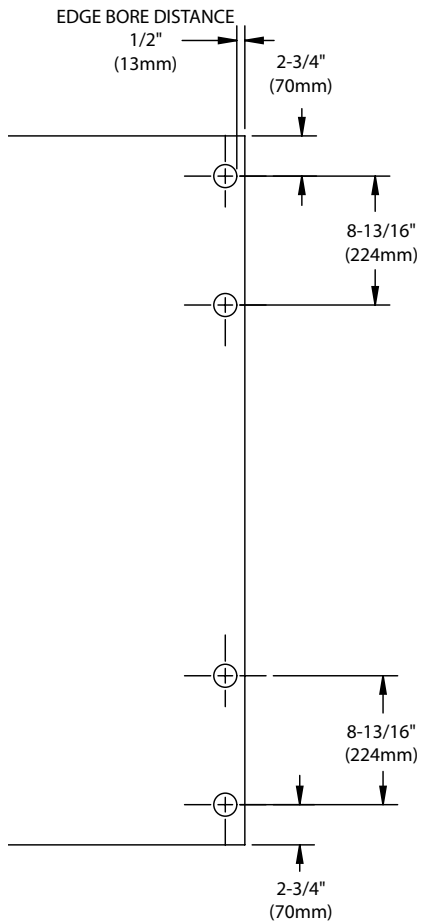
DOOR PREPARATION
