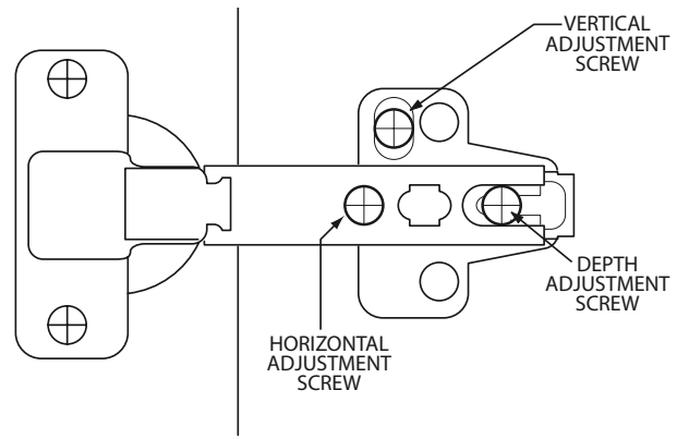
HINGE ADJUSTMENT
