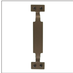
Manija rectangular • 8-5/8" [219.1 mm] x 1-13/16" [46 mm] x 1-1/2" [38.1 mm] HD-RBZ-8 • Bronce pulido (Imagen) HD-RBK-8 • Negro HD-RSN-8 • Niquelado satinado
