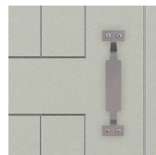
HD-RSN-8 • Manija rectangular con acabado niquelado satinado 8-5/8" [219.1 mm] x 1-13/16" [46 mm] x 1-1/2" [38.1 mm]
